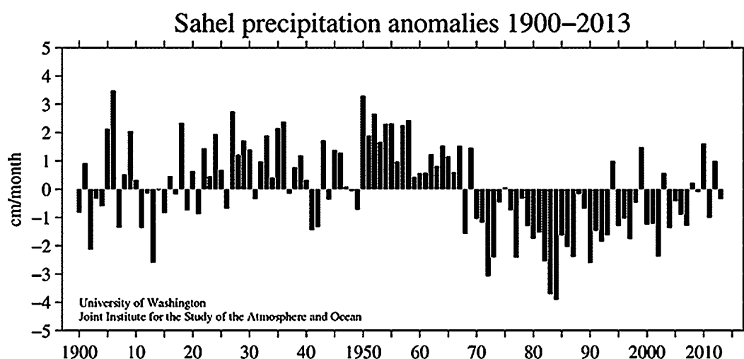
June through October averages over 20–10N, 20W–10E. 1900–2013 climatology NOAA NCDC Global Historical Climatology Network data
